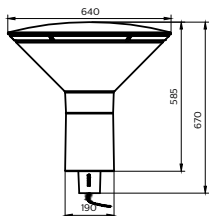
BDS470 CitySpirit Cone Gen2
