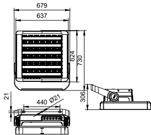
BVP621 LED1110/757 900W AWB PSD GM O
