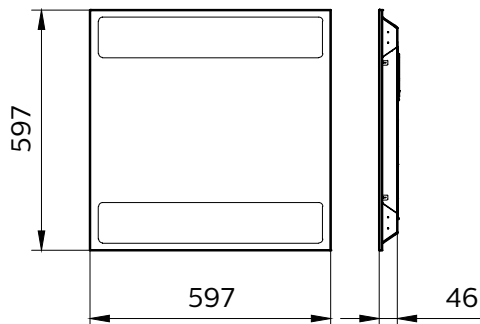
RC100B LED375 865 W603L603 PSD G3
