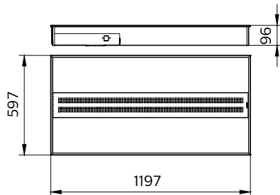
RC420B LED50S/840 PSD W60L120
