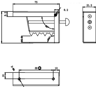
ZGP312 5LED mounting clip GG
