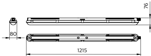
WT198C LED375/840 PSU PCO L1200
