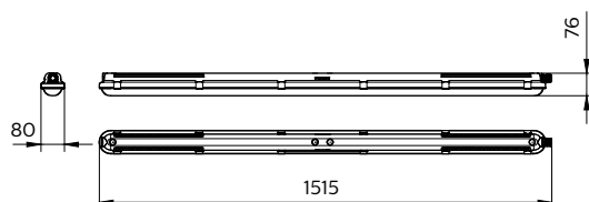
WT198C LED57S/840 PSU PCO L1500
