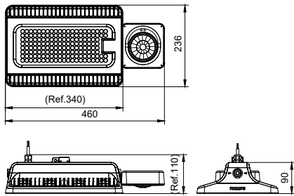
BY570X LED100/CW Connected NB GM
