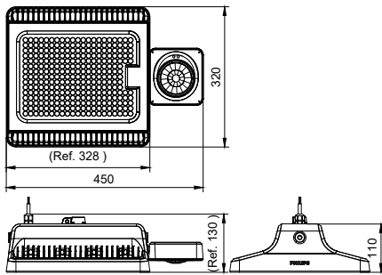
BY570X LED250/CW Connected HRO GM
