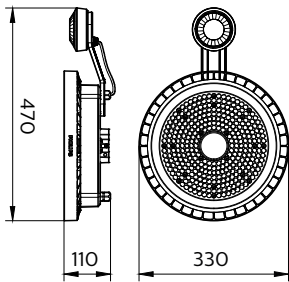
BY698X G5 LED200/NW L1 W WB GM
