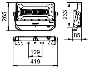
BVP431 LED135/CW 220~240V 100W SWB GM
