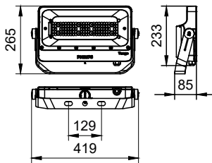
BVP431 LED92/CW 220~240V 70W SMB GM
