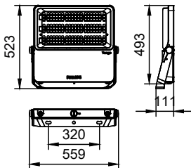
BVP433 LED470/NW 220~240V 345W S6 GM
