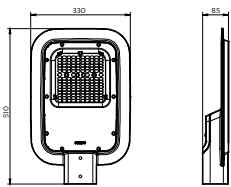
BRP132 LED175/CW 140W 220-240V DM GM
