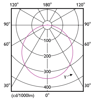
Downlight DN020 G3 CW 10,5W D125 GM
