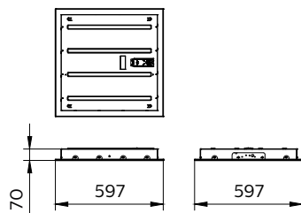
RC650B LED40S965 PSD W60L60
