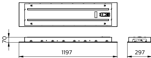
RC650B LED40S965 PSU W30L120
