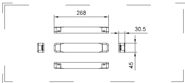
ST307Z 150W 1-10V driver
